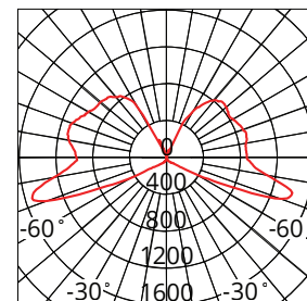
Photometric Diagram
