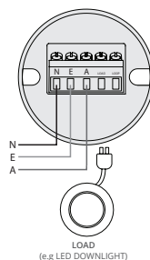
INDIVIDUAL LOAD SMART SINGLE SURFACE SOCKET DIMMER KBSKTD350
