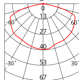
Photometric Diagram
