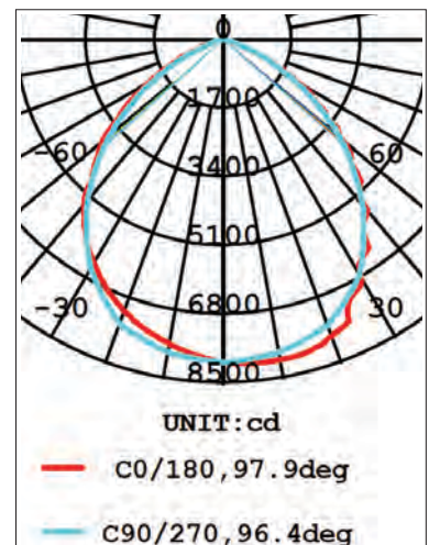
VEGA200W
