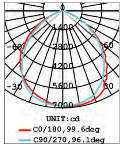
VEGA150W
