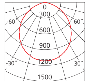
Photometric Diagram
