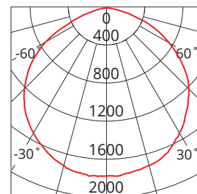
Photometric Diagram
