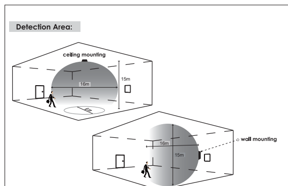
DETECTION AREA
